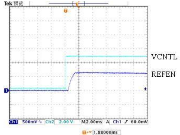
V_{in}=1.5V, V_{OUT}=0.75V, I_{OUT}=1A, V_{CNL}(3.3V) Power-on
